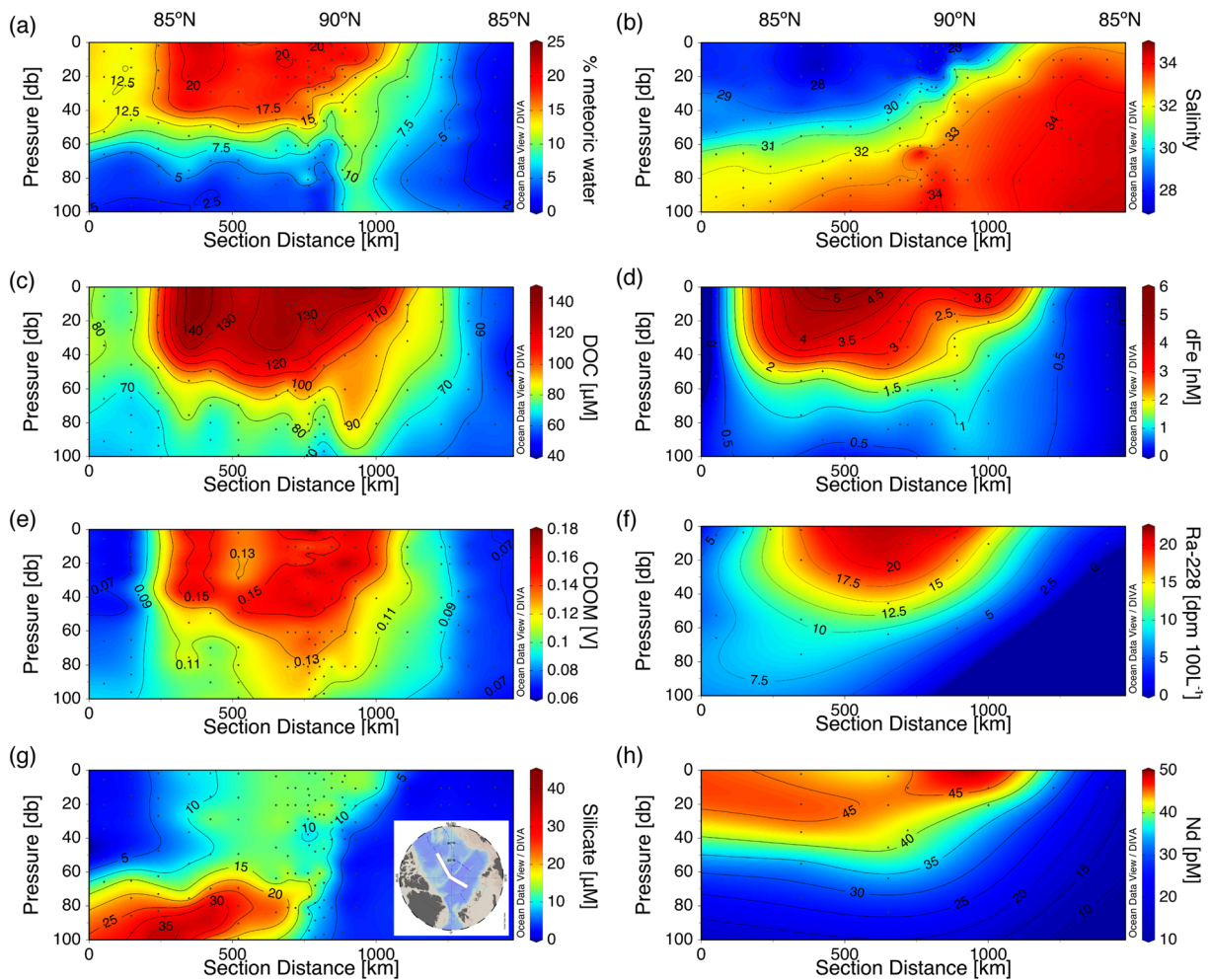
Figure 2. Section plots for (a) % meteoric water, (b) salinity, (c) DOC, (d) dFe, (e) CDOM, (f) ^{228}\text{Ra} , (g) silicate, and (h) dNd along a transect that spans two GEOTRACES cruises and bisects the Transpolar Drift. The stations included in the contour plots is shown on the map inset for (g), and the distance is relative to a station located at 82°N, 150°W.
