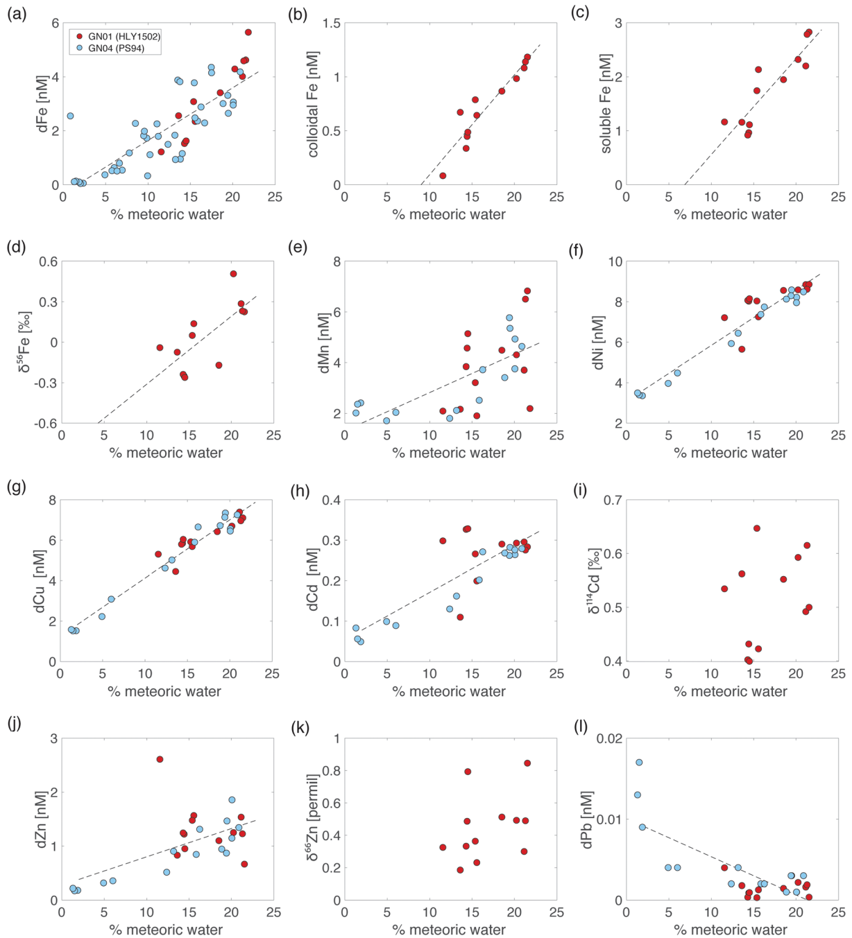
Figure 5. Trace element and isotope concentrations (a) dFe, (b) colloidal Fe, (c) soluble Fe, (d) \delta^{56}\text{Fe} , (e) dMn, (f) dNi, (g) dCu, (h) dCd, (i) \delta^{114}\text{Cd} , (j) dZn, (k) \delta^{66}\text{Zn} , (l) dPb as a function of the meteoric water percentage at stations from the GEOTRACES GN01 (red circles) and GN04 (blue circles) cruises. Data are restricted to 0–50 m for stations north of 84°N. Regression lines are shown for variables with significant ( p < 0.05 ) relationships with meteoric water.
